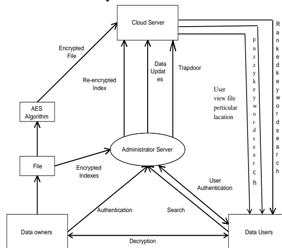
Fig. 1: System architecture
